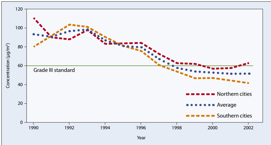
Fig. 10. The development of annual average sulfur dioxide concentrations in Chinese cities from 1990 to 2002
