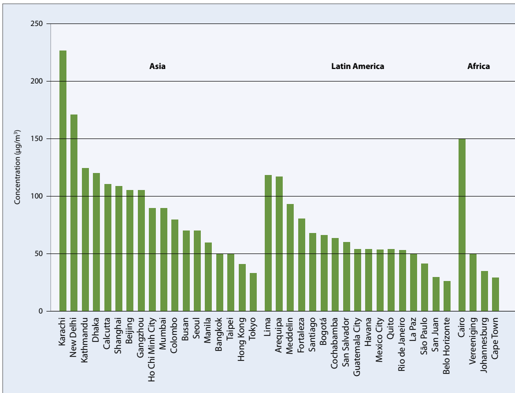
Fig. 4. Annual average PM 10 concentrations observed in selected cities worldwide
