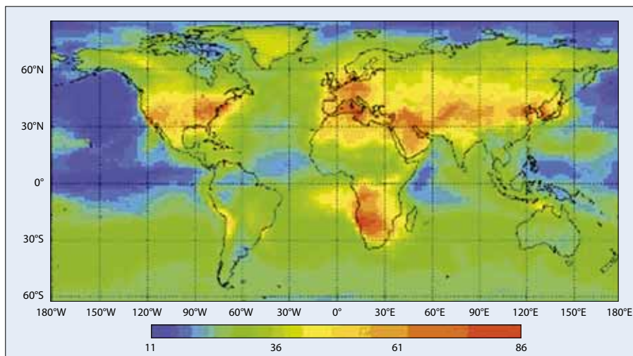
Fig. 5. Mean afternoon (13:00 to 16:00) surface ozone concentrations calculated for the month of July
