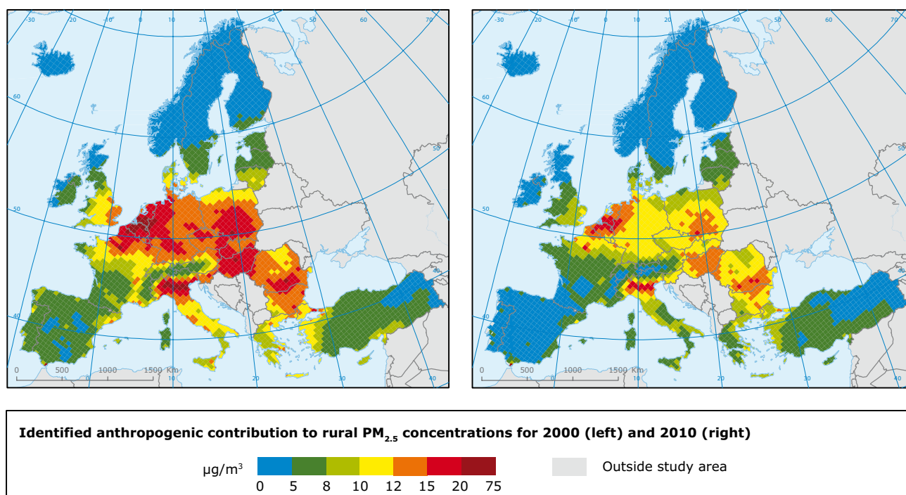
Figure 3.22 Identified anthropogenic contribution to rural PM 2.5 concentrations (annual mean, µg/m 3 ) for 2000 and 2010, for CAFE baseline emissions; using four-year average meteorological conditions
