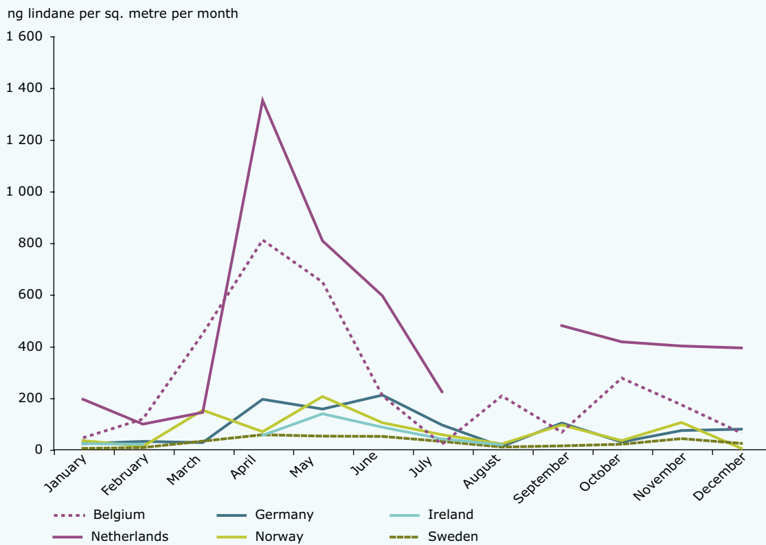
Figure 4.10 Observed coastal lindane deposition, 2003
