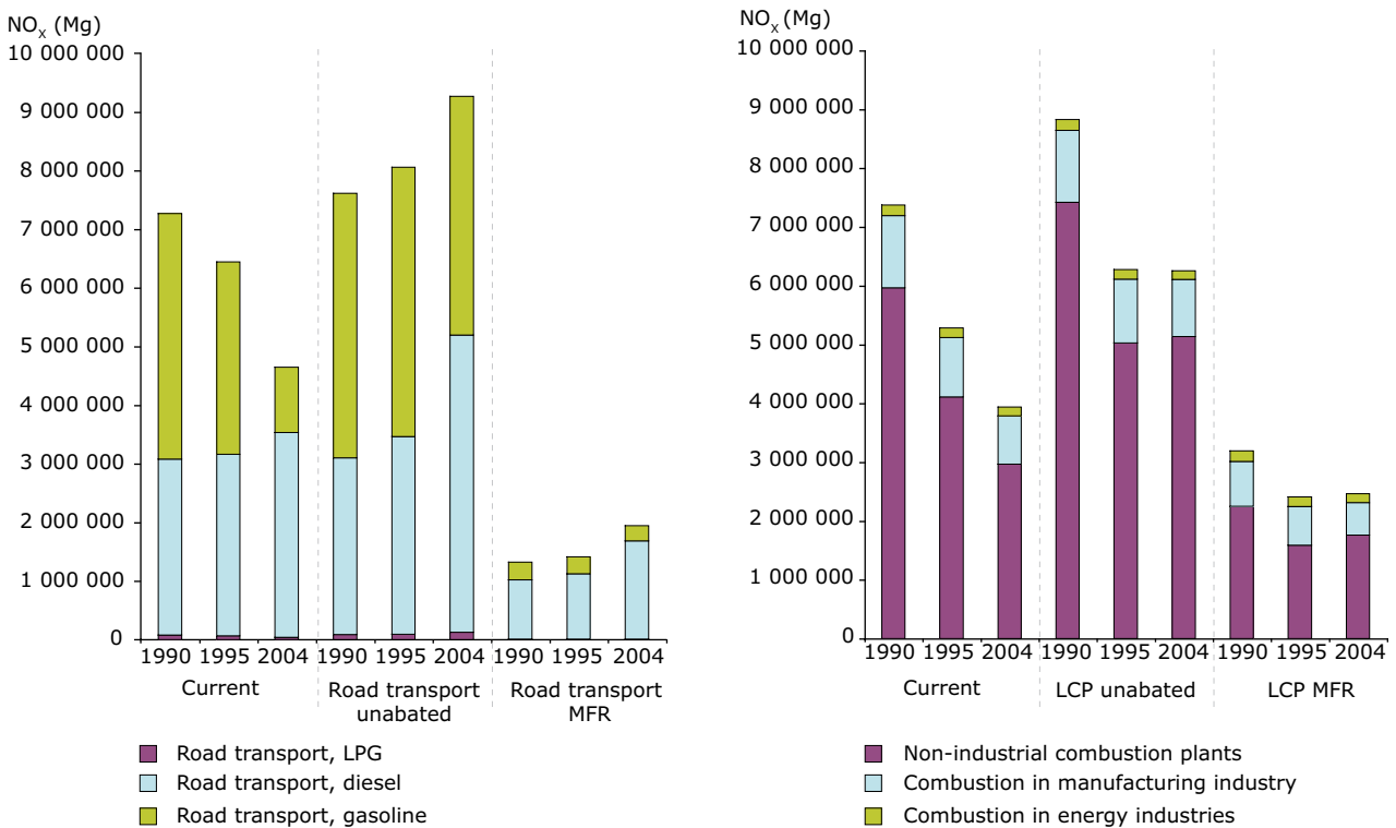
Figure 3.30 The effect in the EU-25 of introducing vehicle emission standards in road transport (left) and emission abatement at large combustion plants (right) on the emission of NO x
