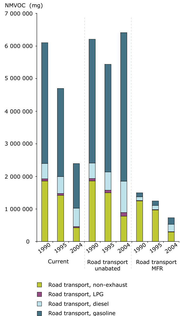
Figure 3.8 The effect (for EU-25) of introducing vehicle emission standards in road transport on the emission of NMVOC
